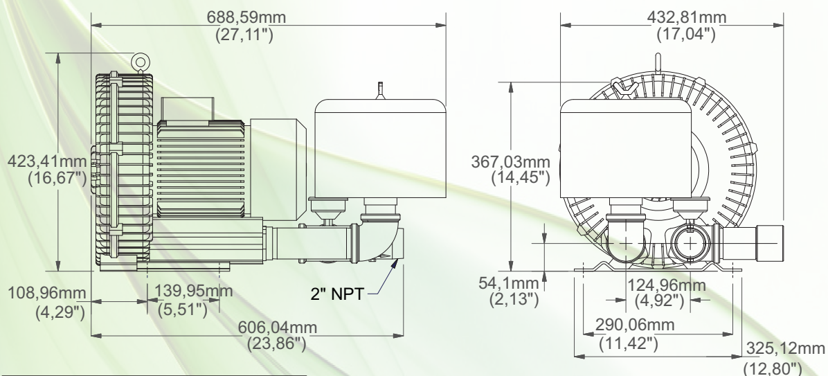
Kit Pressure Pump 2" NPT KPPB-600
