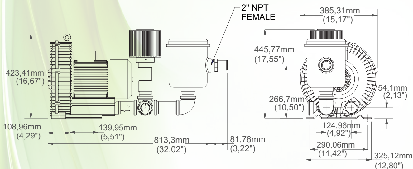
Kit Vacuum Pump 2" NPT KVPB-600
